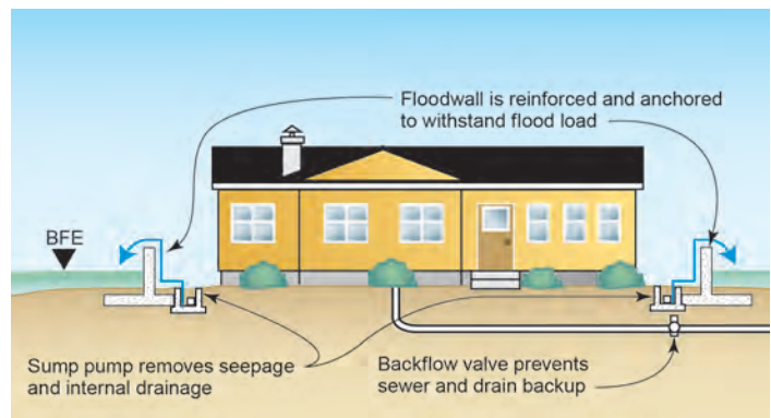
Figure 9: Residential floodwall
