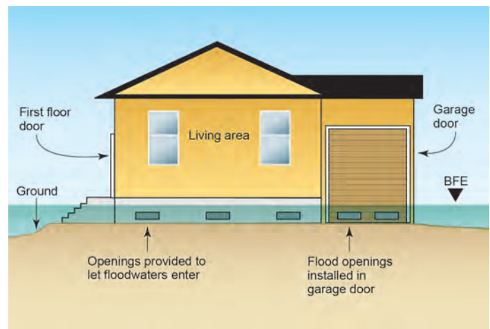
Figure 4: Flood openings and their placement
