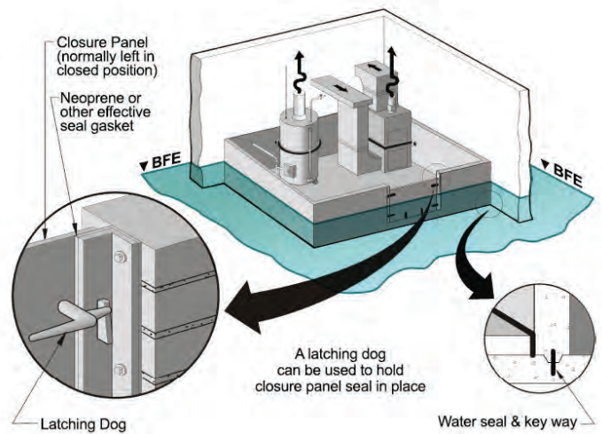
Figure 6: Detail of floodproofed building utility
